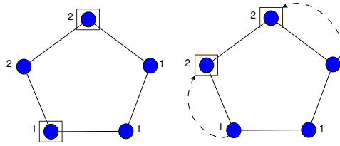
FIGURE 1. Left: a maximum weighted minimal dominating set ( \Gamma_w(G) = 3 ). Right: a maximum weighted irredundant set ( IR_w(G) = 4 ), where the dashed arrows link vertices of the irredundant set to their private vertices.
