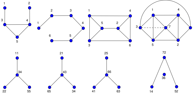
FIGURE 3. A claw in \text{bull}' , P_6' and \overline{C_6}' , and a co-paw in G_1^{7'} and G_2^{7'} (note that G_1^{7'} and G_2^{7'} only differ in the edge (3, 7) , which is displayed here by a dashed line).
