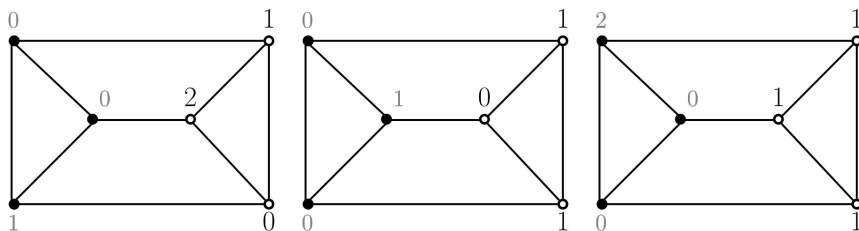
FIGURE 5. Extension of the coloring of G' when the edge e is of type 1.
