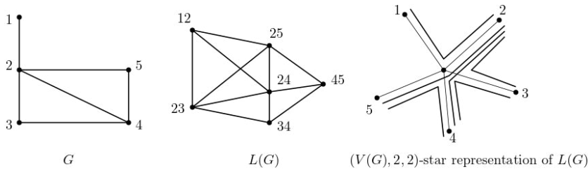
FIGURE 1. Example of the construction of an EPT-star representation of L(G)
