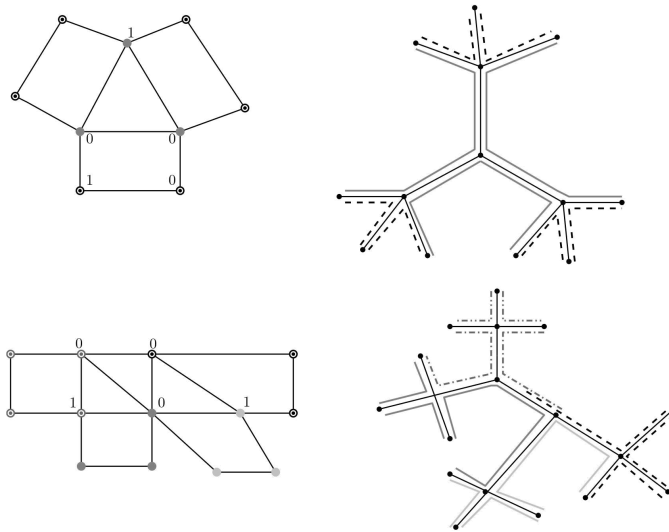
FIGURE 6. Examples of [4, 2, 2] -graphs which are not 2-clique colorable.
