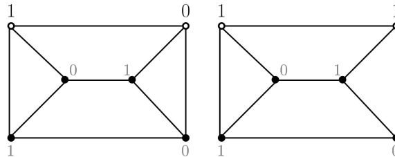
FIGURE 4. Extension of the coloring of G' when the edge e is of type 2.
