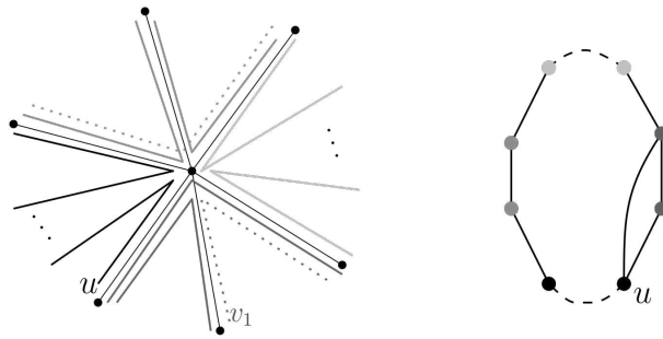
FIGURE 2. Construction of G' . The dotted paths correspond to the vertices that are removed.
