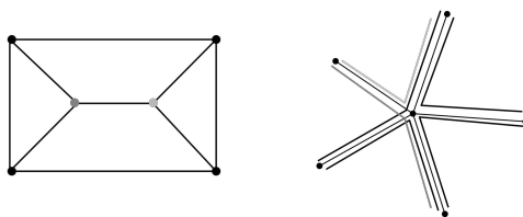
FIGURE 3. Prism graph and its EPT representation
