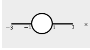
FIGURE 15. Domain \Omega = \mathbb{C} \setminus \left( \overline{B(0, 1)} \cup [-3, -1] \cup [1, 3] \right) with basepoint z_0 = 4 .
