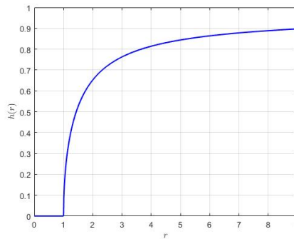
FIGURE 2. Graph of h -function for exterior of parabola y^2 = -4x with basepoint z_0 = 1 .
