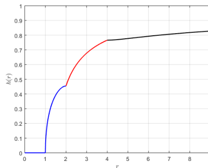
FIGURE 14. Graph of h -function for domain \Omega = \mathbb{C} \setminus \left( \overline{B(0,1)} \cup [1,2] \cup (-\infty, -1] \right) with basepoint z_0 = 3 .
