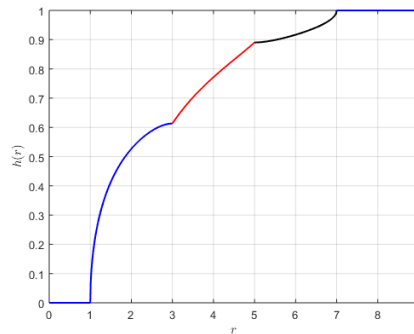
FIGURE 16. Graph of h -function for domain \Omega = \mathbb{C} \setminus (\overline{B(0,1)} \cup [-3, -1] \cup [1, 3]) with basepoint z_0 = 4 .
