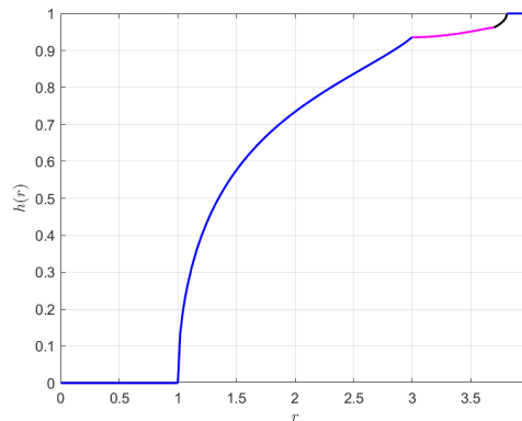
FIGURE 18. Graph of h -function for domain \Omega = \mathbb{C} \setminus (\{|z| \leq 1\} \cup [1, 1.700005] \cup \{|z - 1.755190| \leq 0.055185\}) with basepoint z_0 = -2 .
