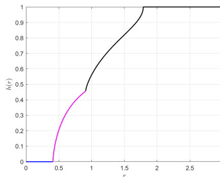
FIGURE 7. Graph of h -function for domain \Omega = B(0, 1) \cup B(1.5, 1) with basepoint z_0 = 0.75 + 0.25i .
