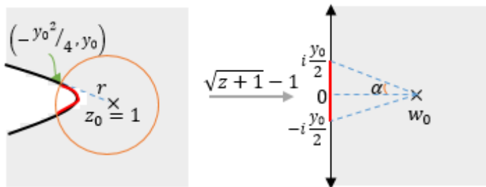
FIGURE 1. Conformal transformation from exterior of parabola to halfplane. The set E_r (left) and its image f(E_r) (right) are shown in red.
