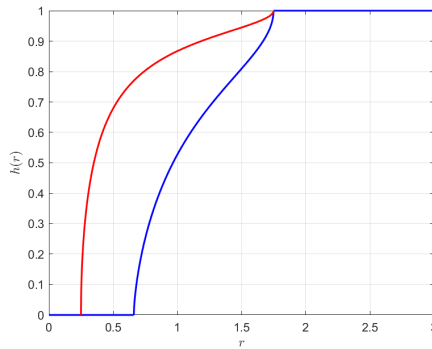
FIGURE 6. Comparing the graphs of h -function for the interior of the unit disc (red) and the domain \Omega = B(0, 1) \cup B(1.5, 1) with same basepoint z_0 = 0.75 (blue).
