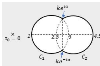
FIGURE 3. Domain \Omega = \mathbb{C} \setminus (\overline{B(2,1)} \cup \overline{B(3.5,1)}) with various positions of basepoint z_0 .
