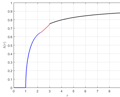
FIGURE 10. Graph of h -function for round lollipop domain \Omega = \mathbb{C} \setminus (\overline{B(0, 1)} \cup (-\infty, -1]) with basepoint z_0 = 2i or z_0 = -2i .
