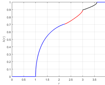
FIGURE 12. Graph of h -function for finite lollipop \Omega = \mathbb{C} \setminus (\overline{B(0, 1)} \cup [1, 3]) with basepoint z_0 = 2i .
