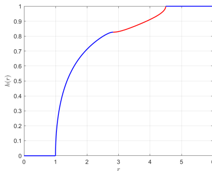
FIGURE 4. Graph of h -function for domain \Omega = \mathbb{C} \setminus \left( \overline{B(2, 1)} \cup \overline{B(3.5, 1)} \right) with basepoint z_0 = 0 .
