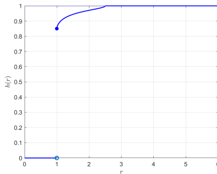
FIGURE 8. Graph of h -function for domain \Omega = B(0, 1) \cup B(1.5, 1) with basepoint z_0 = 0 .
